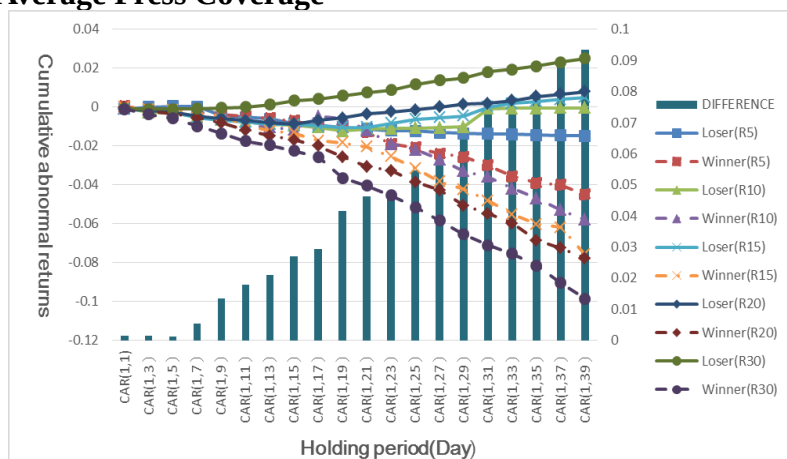
Figure 2 Comparison of CAR (Cumulative Abnormal Returns) between High and Low Press Coverage
